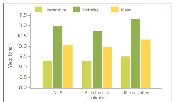
Figure 20. The benefit of little and often sulphur (Winter Wheat, 2000)
