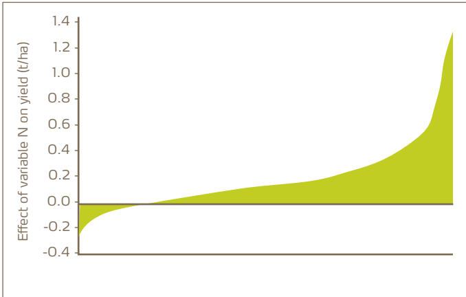
Figure 27. Yield advantage with the N-Sensor. (1999-2005, 186 trials)
