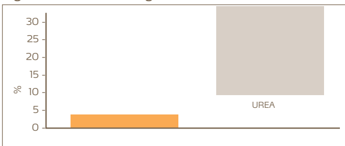
Figure 13. Loss of Nitrogen as ammonia
