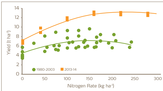
Figure 12. Nitrogen Dose response trials
