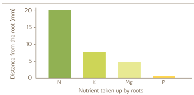
Figure 23. Distance of nutrient uptake by roots
