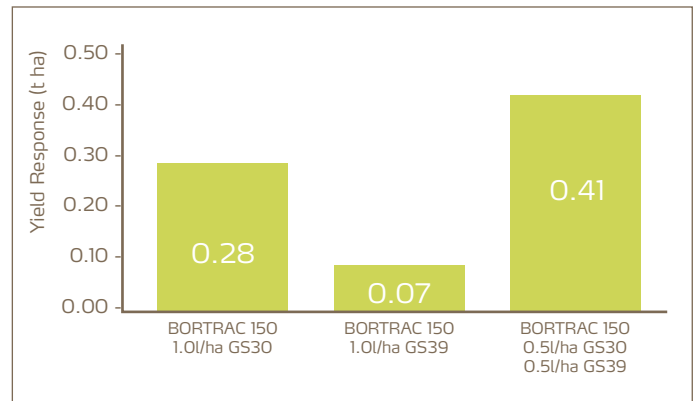
Figure 5. Yield Response of Winter Wheat to Boron
