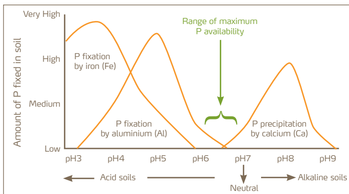
Figure 3. Influence of soil pH on the soil P availability
