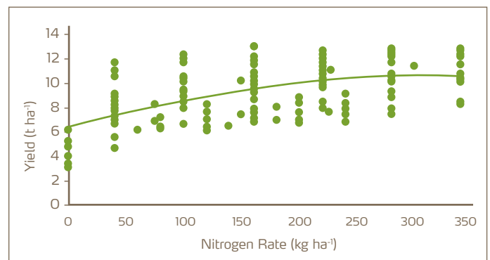
Figure 11. Nitrogen Dose response trials
