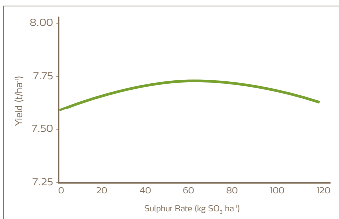
Figure 18. Optimum Sulphur rates (Winter Wheat)
