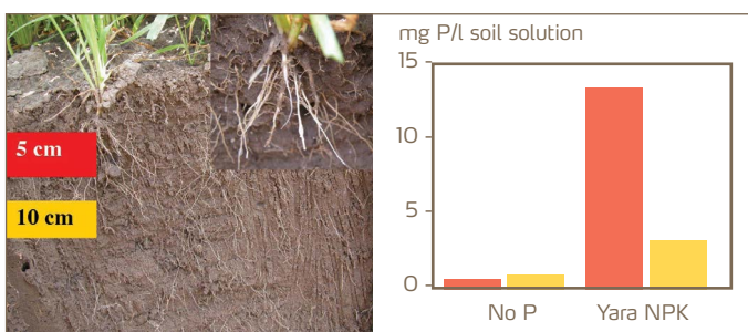
Figure 22. Phosphate in soil solution
